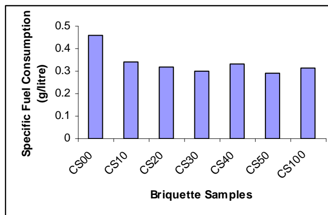
Figure 7. Results of specific fuel consumption
