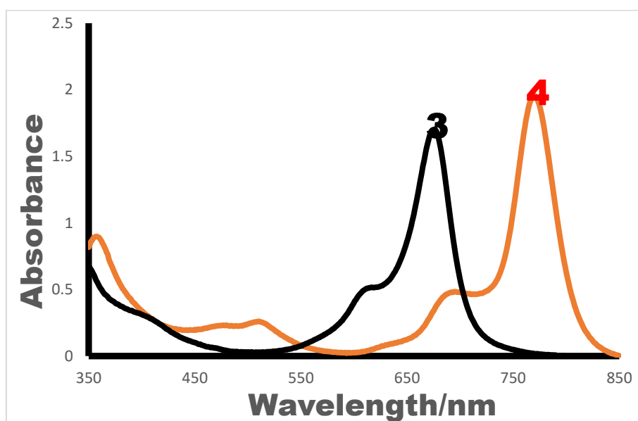
Figure 2. UV-Vis spectra of complexes 3 ( 2.41 \times 10^{-6} M) and 4 ( 2.42 \times 10^{-6} M) in DMF
