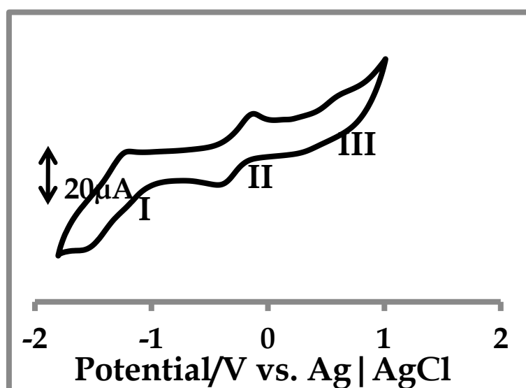
Figure 3. Cyclic voltammetry profiles of 1 \times 10^{-4} M 1 \times 10^{-4} M of cobalt 4-(2-aminoethylthio) phthalocyanine in freshly distilled DMF containing 0.1 M TBABF 4 supporting electrolyte. Scan rate: 100 \text{ mVs}^{-1} 100 \text{ mVs}^{-1}
