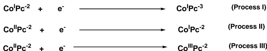
Figure 4. Redox processes I, II and III for Cobalt 4-(2-aminoethylthio) phthalocyanine complex
