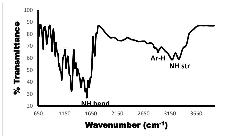
Figure 1. FTIR spectrum representative of compound 4
