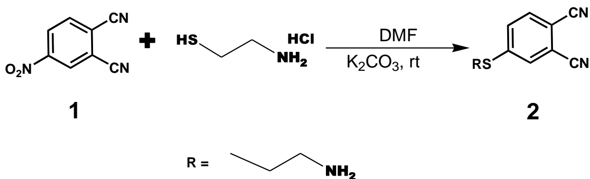
Scheme 1. Synthetic pathway for the synthesis of 4-(2-aminoethylthio) phthalonitrile (2)
