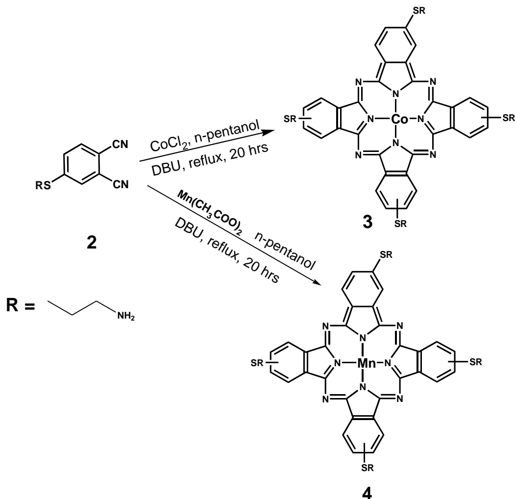
Scheme 2. Synthetic pathway for the formation of 4-(2-aminoethylthio) phthalocyanine Cobalt (II), 3 , and Manganese (III), 4
