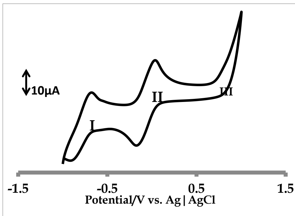
Figure 4. Cyclic voltammery profiles of 1 \times 10^{-4} M 1 \times 10^{-4} M of Manganese 4-(2-aminoethylthio) phthalocyanine complex in freshly distilled DMF containing 0.1 M TBABF 4 supporting electrolyte. Scan rate: 100 \text{ mVs}^{-1} / 100 \text{ mVs}^{-1}
